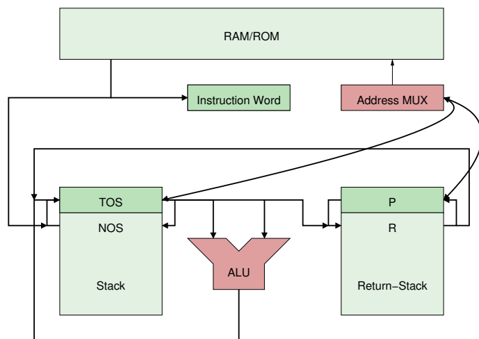
Figure 1: Block Diagram
